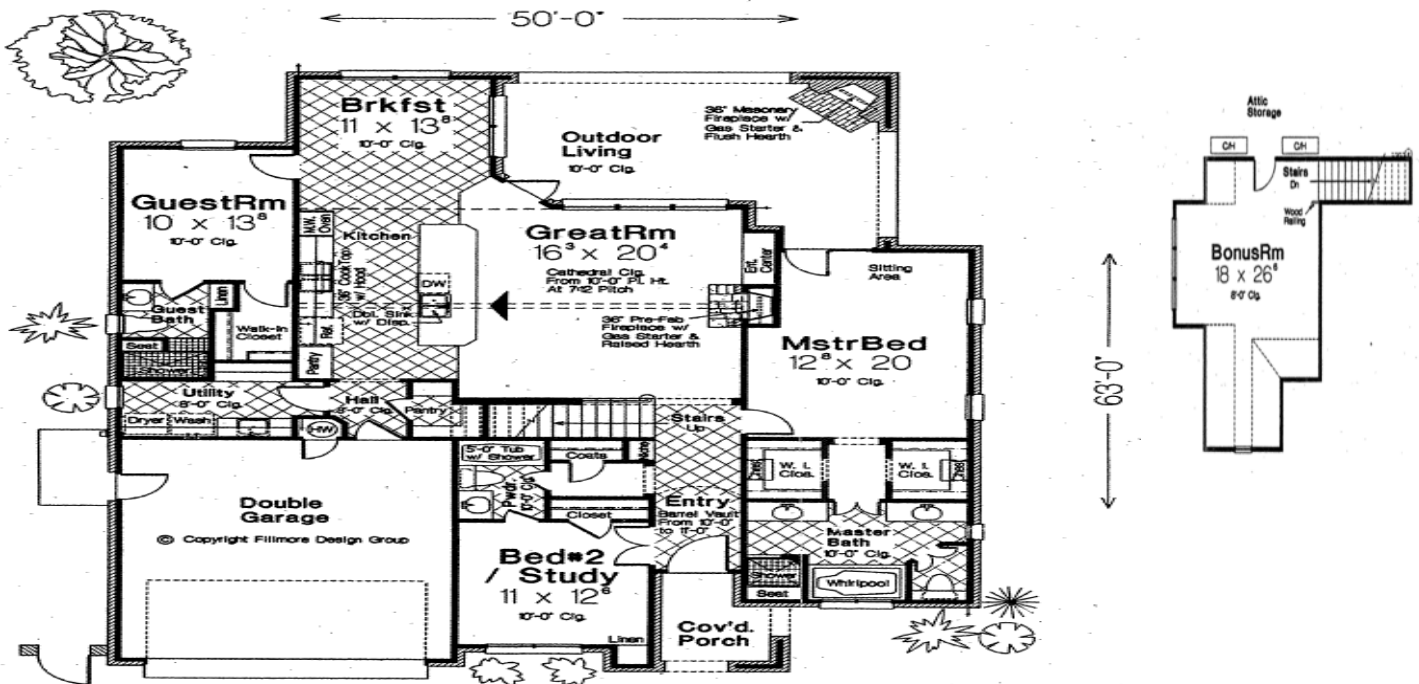
Lower Level Floor Plan 2021 Sq. Ft. First Floor Heated & Cooled Areas Only
