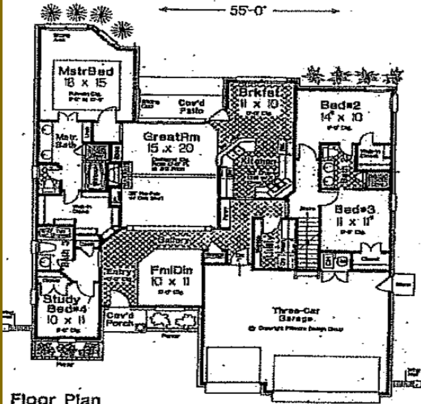
Floor Plan 2255 Sq. Ft. 1st Floor Only
